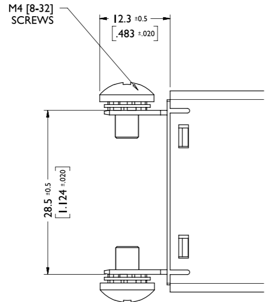
SCREW TERMINAL
