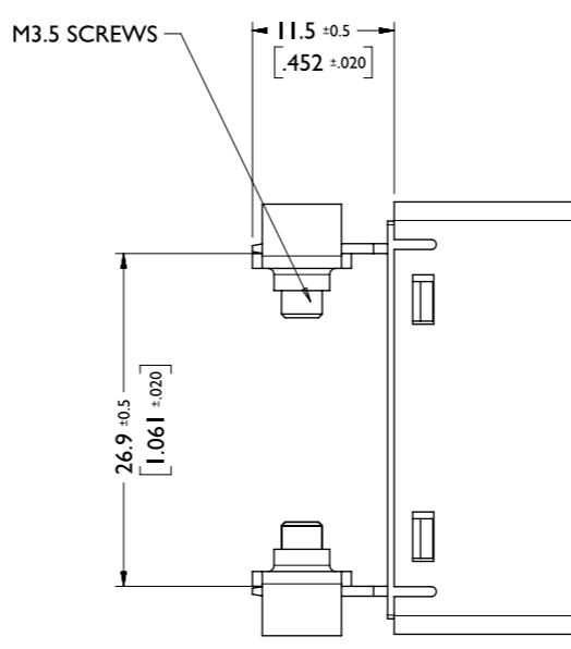
CLAMP TERMINAL
